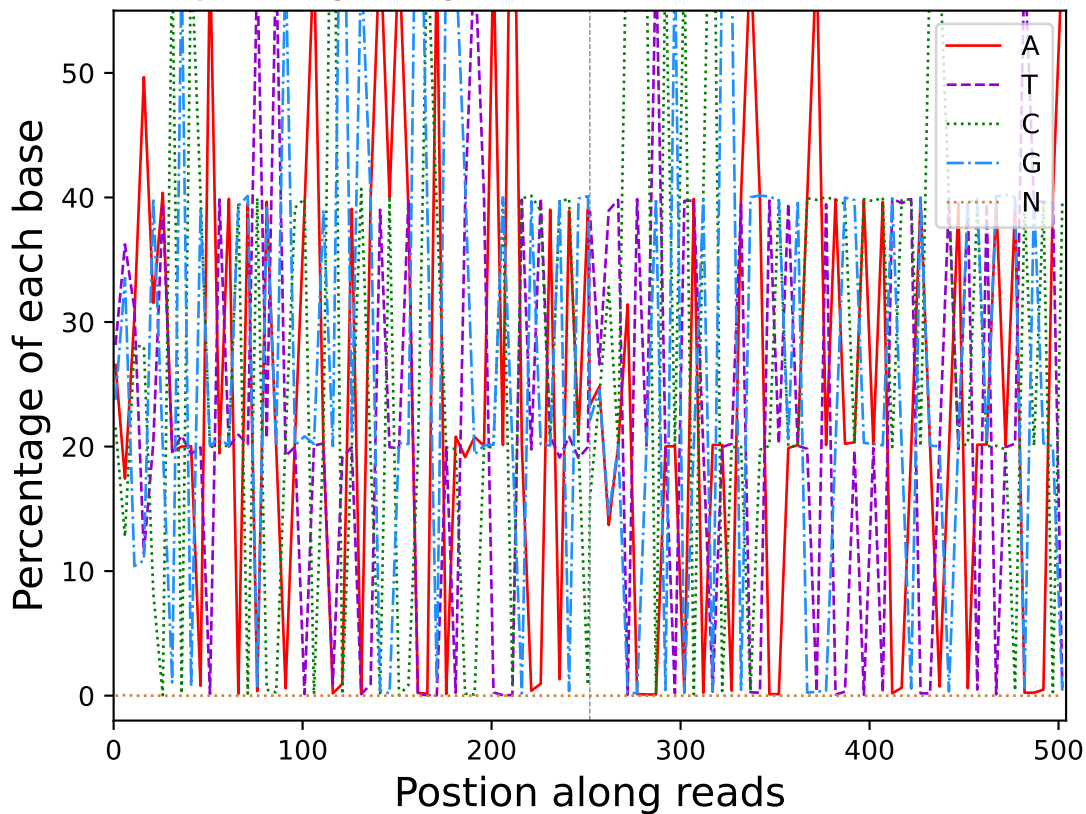
Base percentage along reads (R10820)
